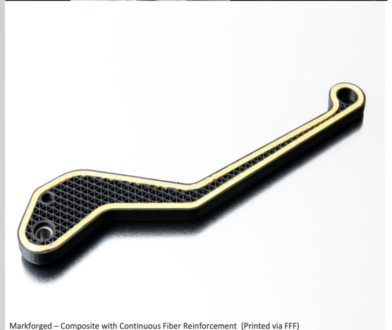
Markforged – Composite with Continuous Fiber Reinforcement (Printed via FFF)
